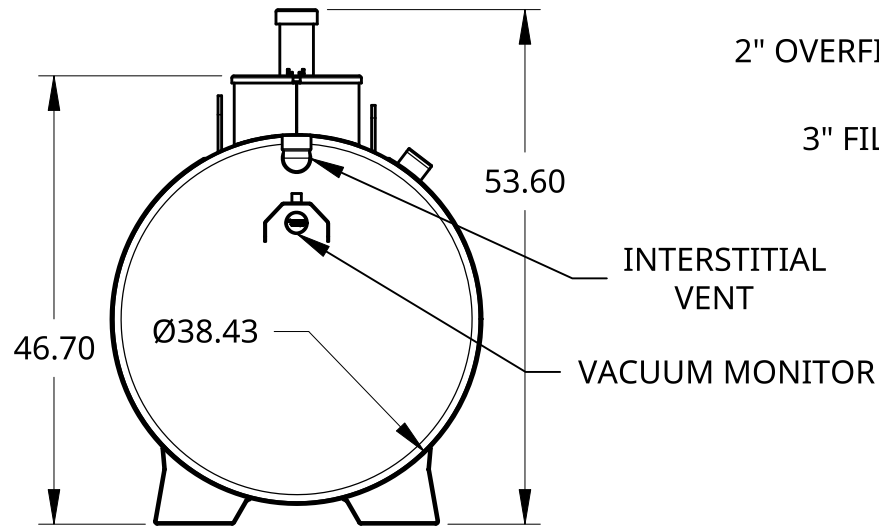
FRONT VIEW
